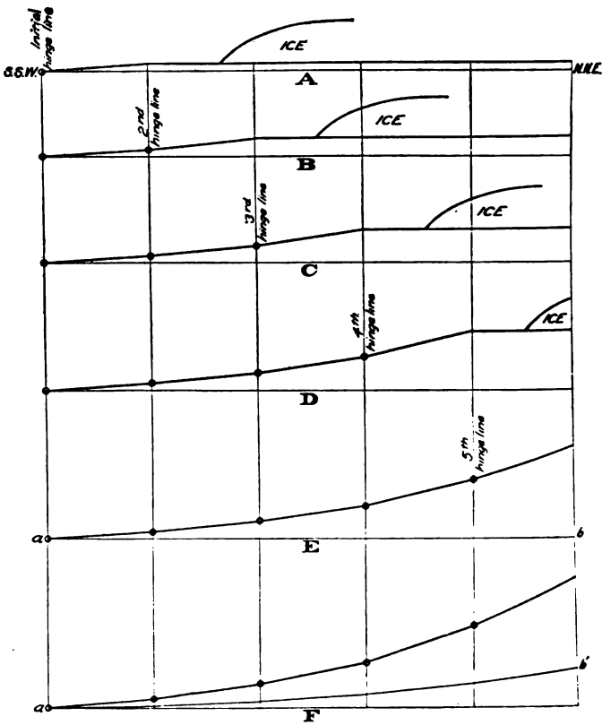
FIG. 375. — Series of idealistic diagrams to indicate the nature of the quick recovery of the crust by uplift in blocks unloaded of the ice in succession. A further slower uplift, added after the completion of the first movement, is brought out in the last diagram (b').
